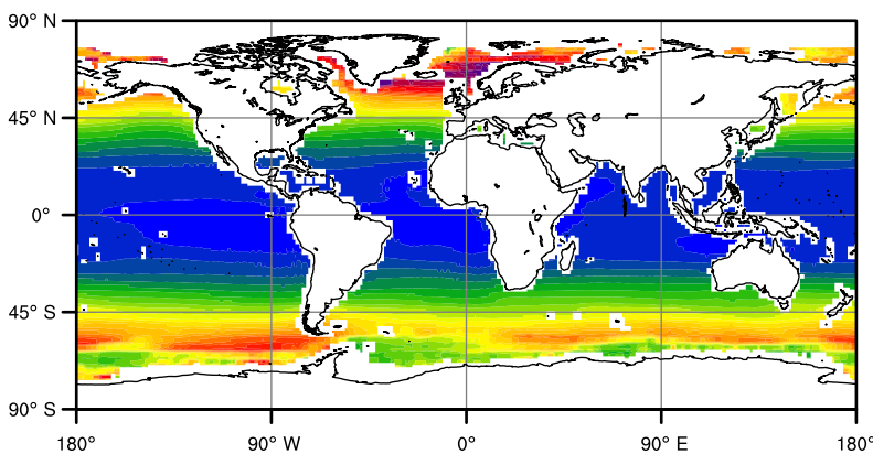
(e) Model ARPEGE-new
