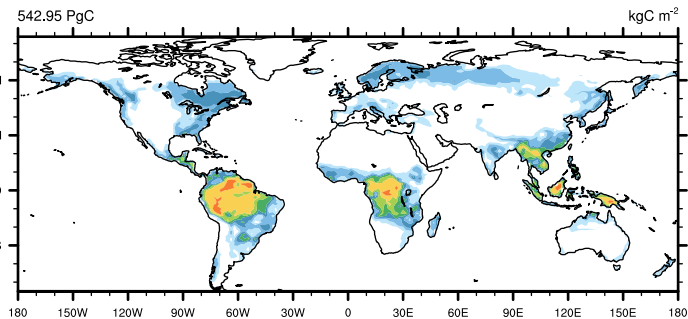
S_{\text{All}} C_{\text{veg}} JULES-C2
