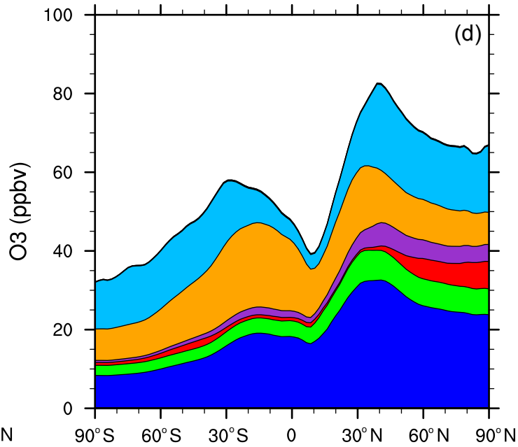
400 hPa - July 2010
