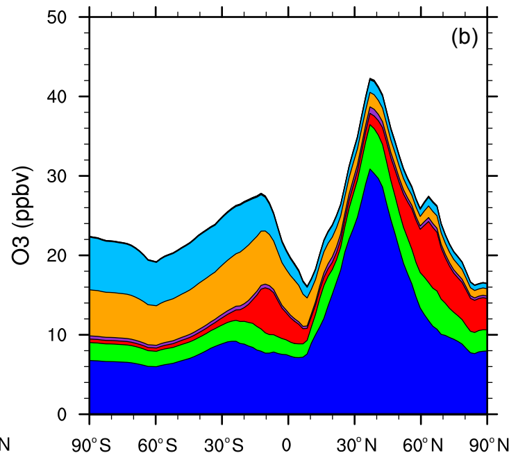
400 hPa - July 2010
