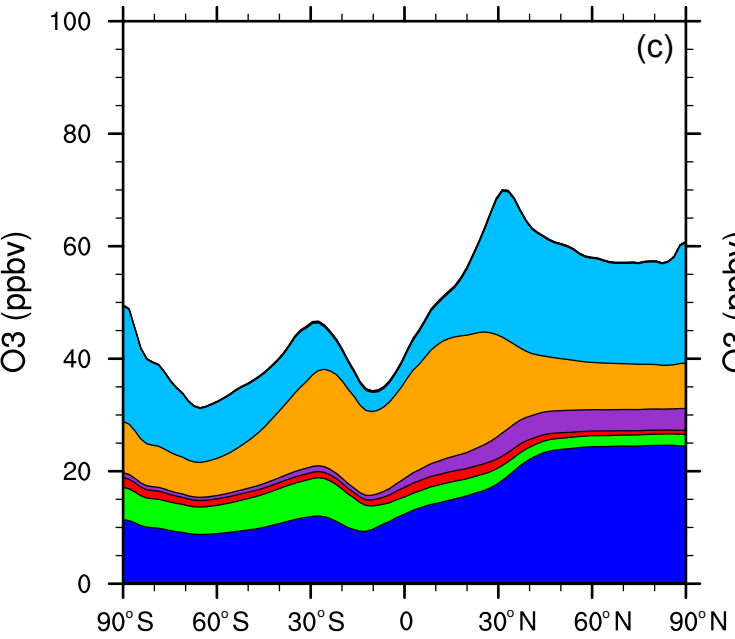
400 hPa - January 2010
