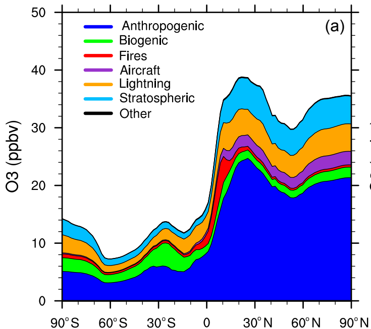
400 hPa - January 2010
