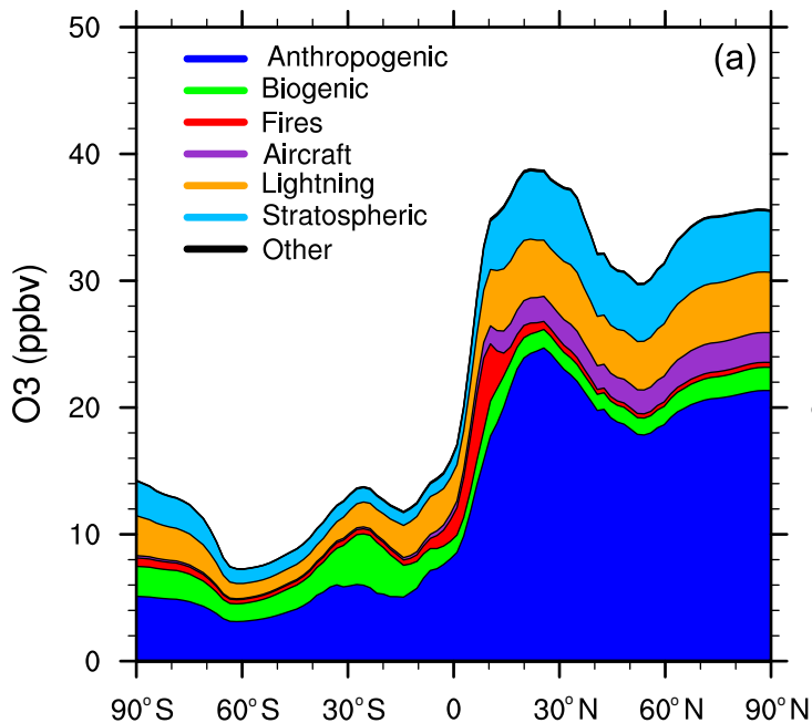
400 hPa - January 2010
