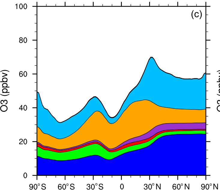
400 hPa - January 2010
