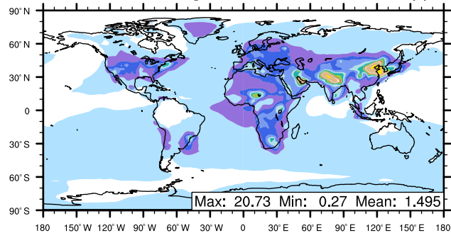
O3_X_ANT mixing ratio ppb
