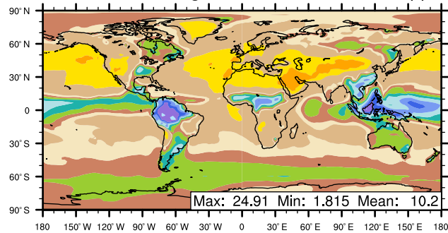
O3_X_BIO mixing ratio ppb
