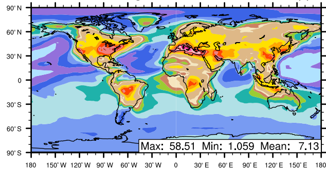
O3_X_STR mixing ratio ppb
