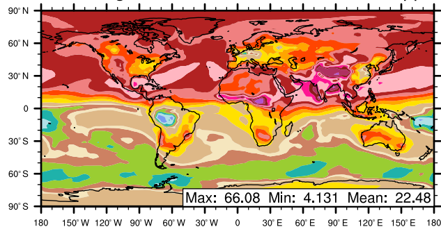
O3_X_ANT mixing ratio
