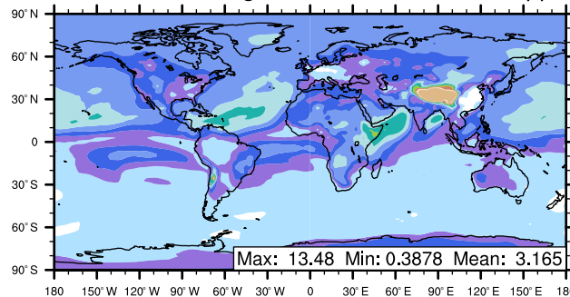
O3_X_BIO mixing ratio
