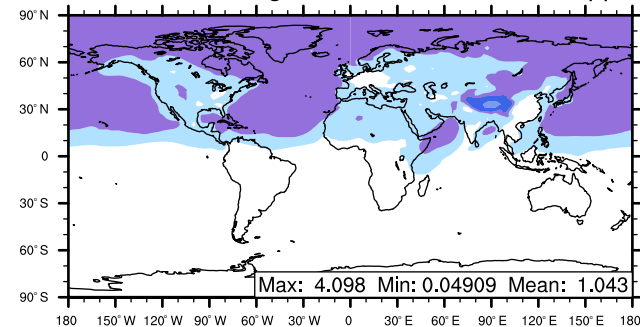
O3_X_BMB mixing ratio
