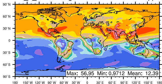
O3_X_ANT mixing ratio
