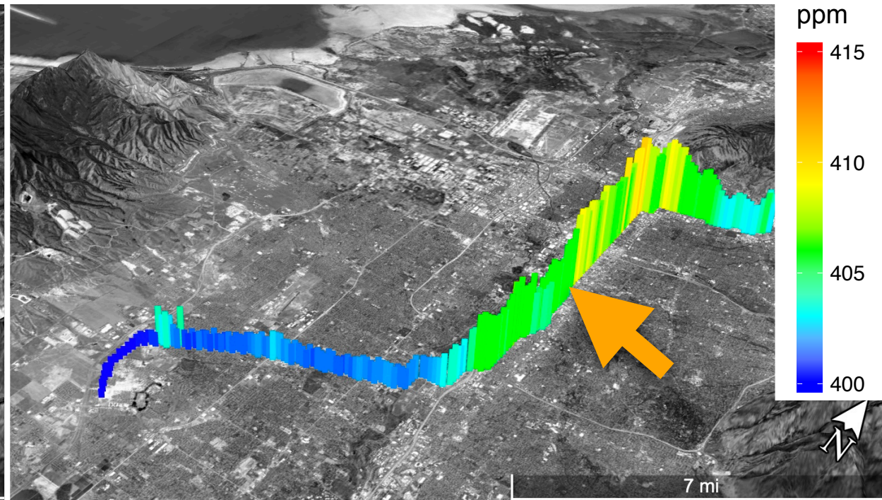
Modeled CO 2 mole fraction
