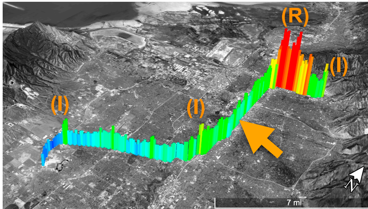
Measured CO 2 mole fraction
