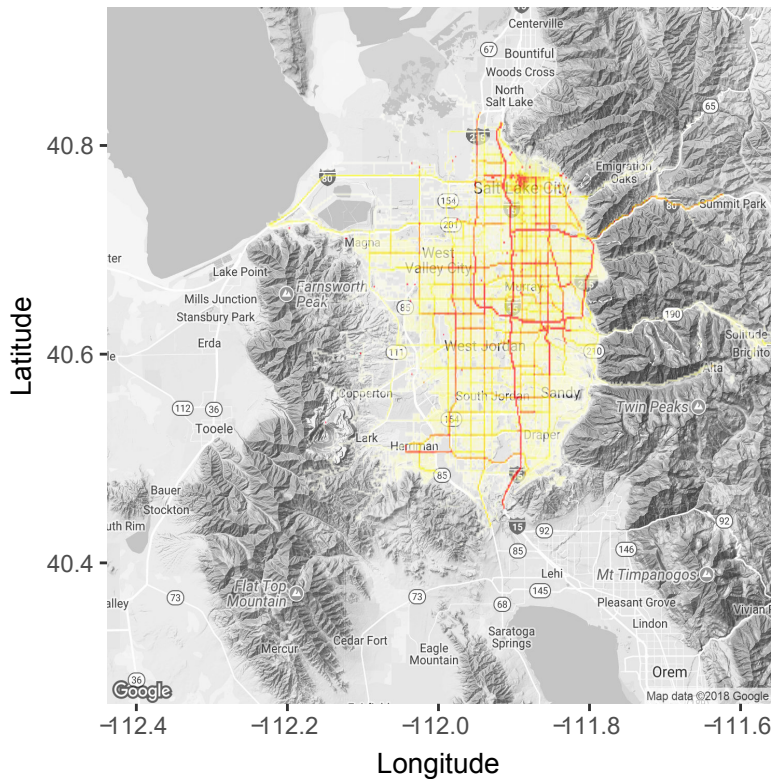
STILT footprint
