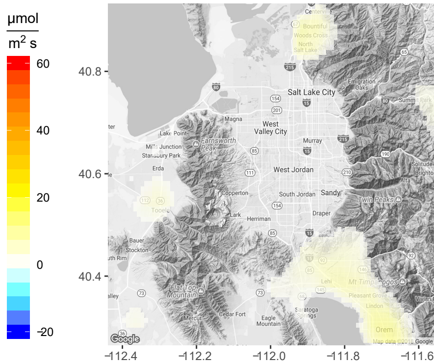
ODIAC emission inventory
