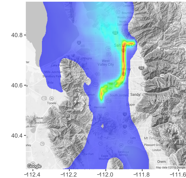
STILT footprint
