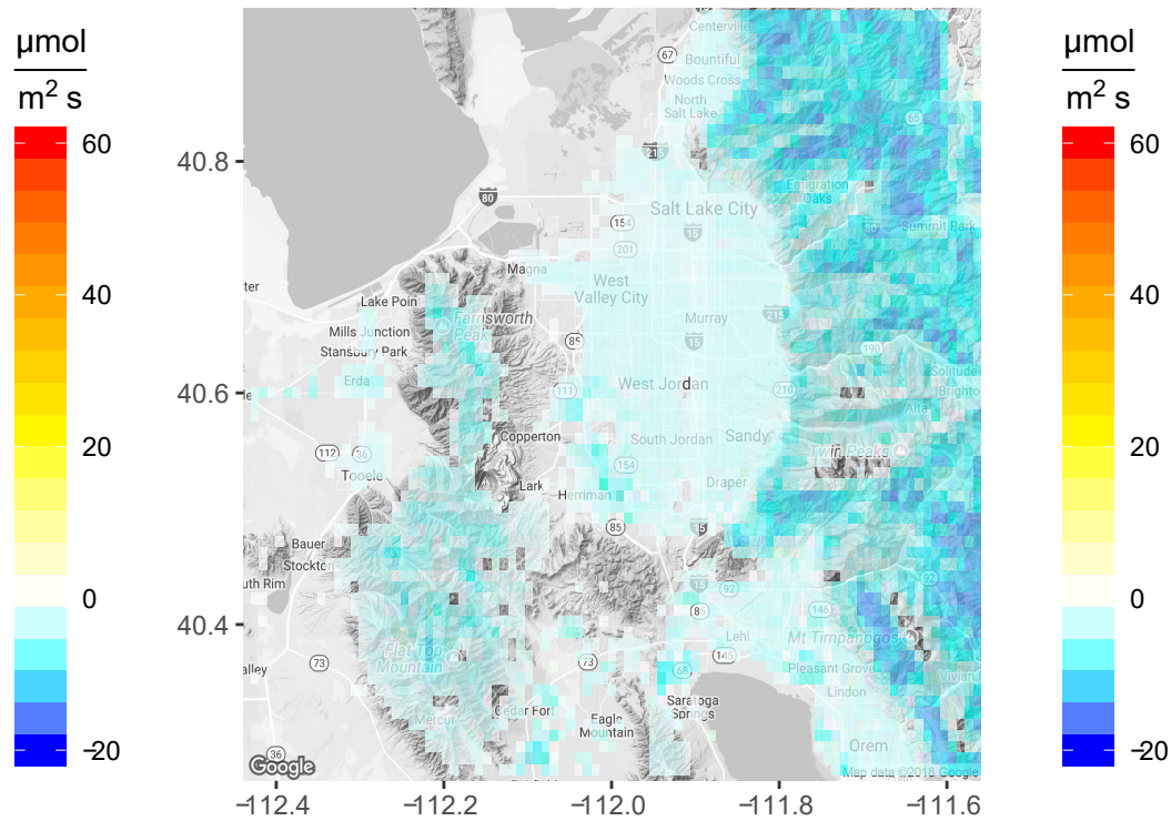
Biological flux inventory
