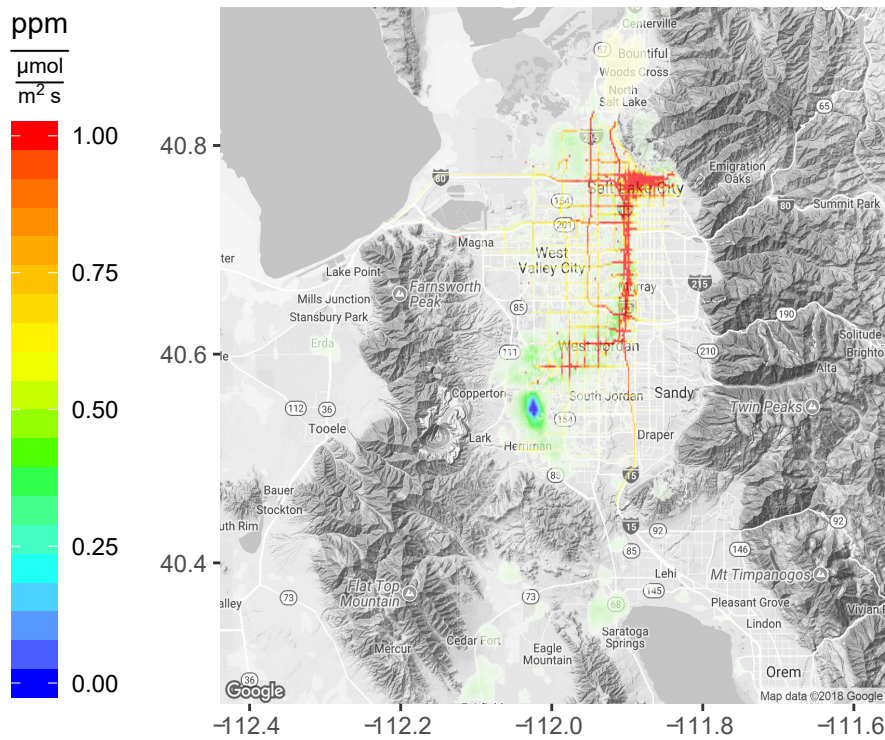
Mean modeled CO 2 contribution
