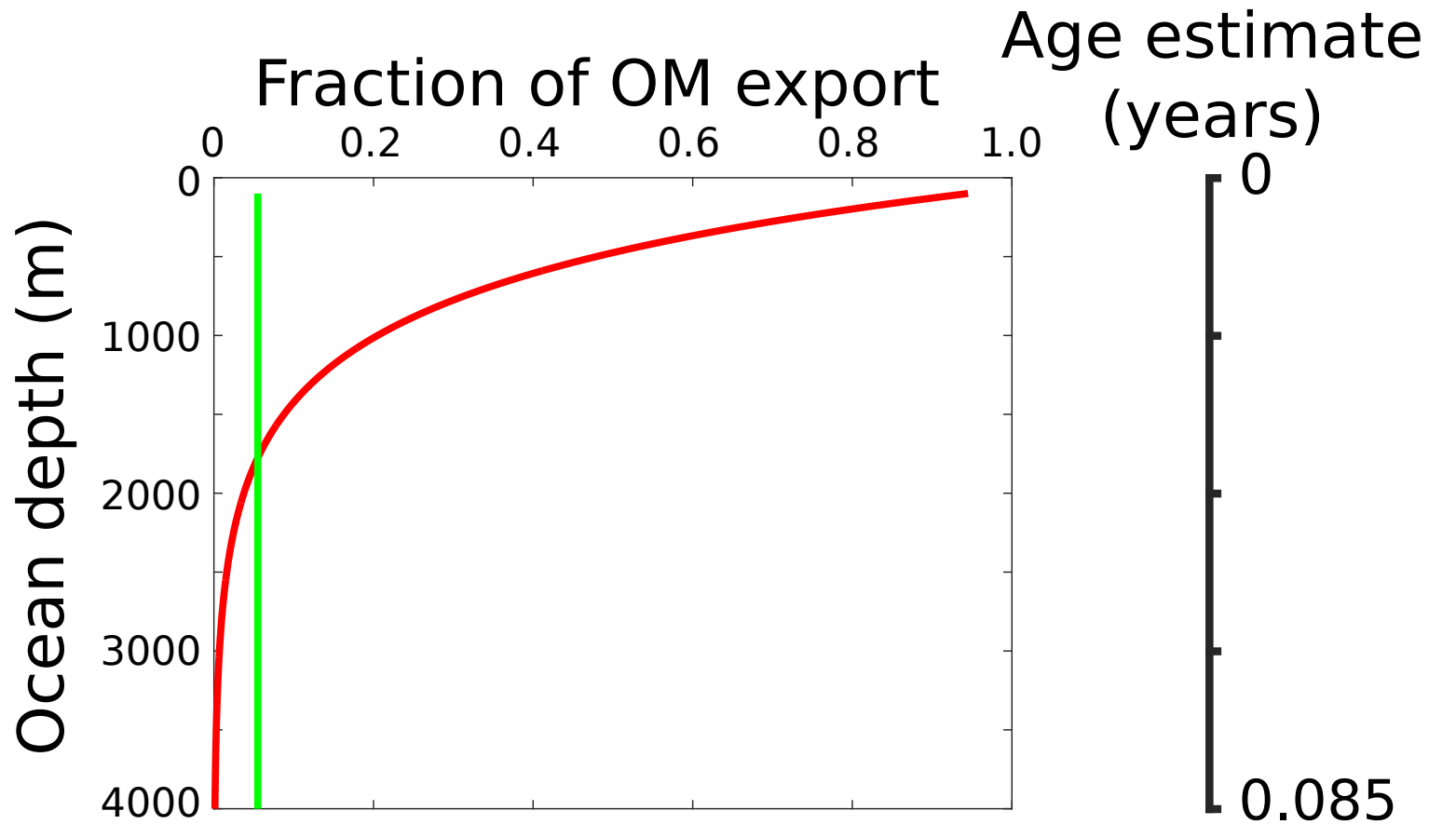
(b) Deep ocean (4000 m)
