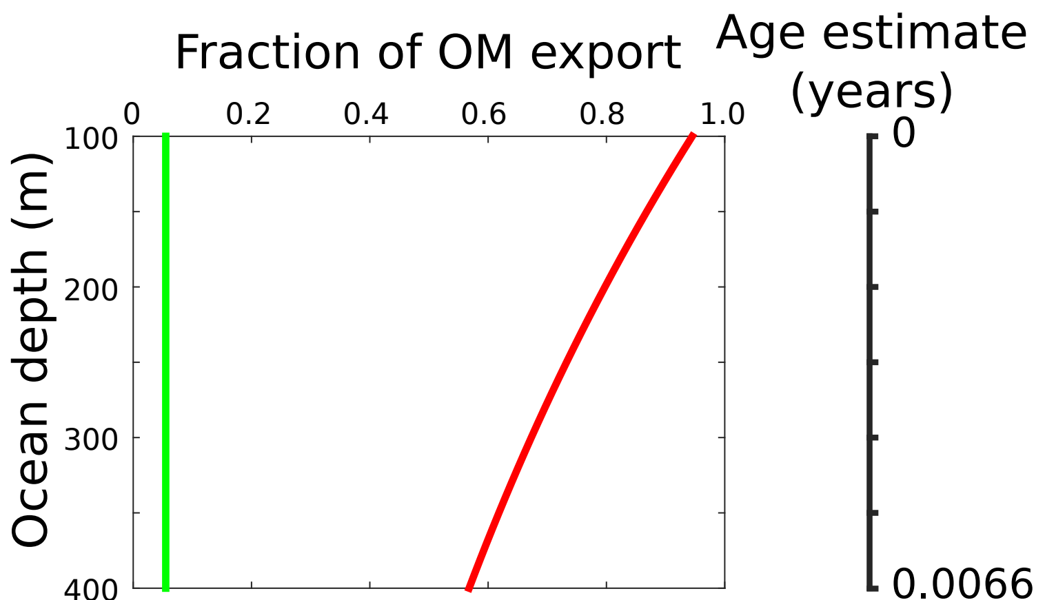
(a) Shallow ocean (400 m)
