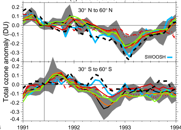
(b) Ozone at 20–70 hPa
