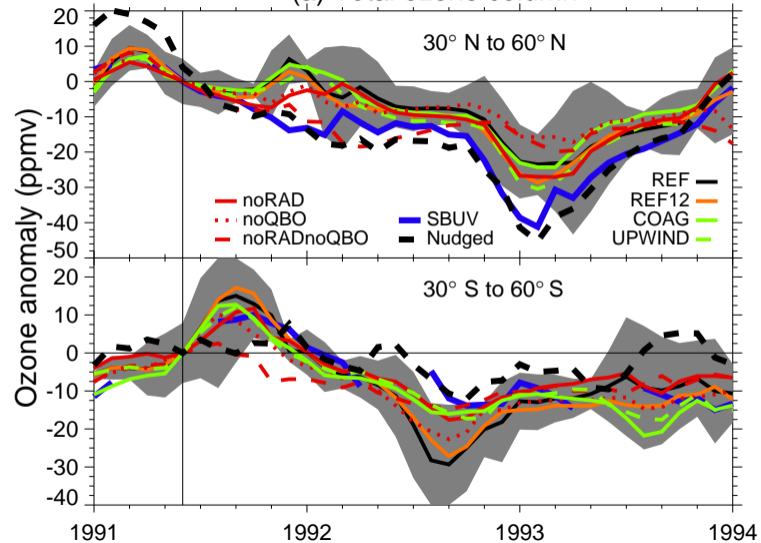
(a) Total ozone column
