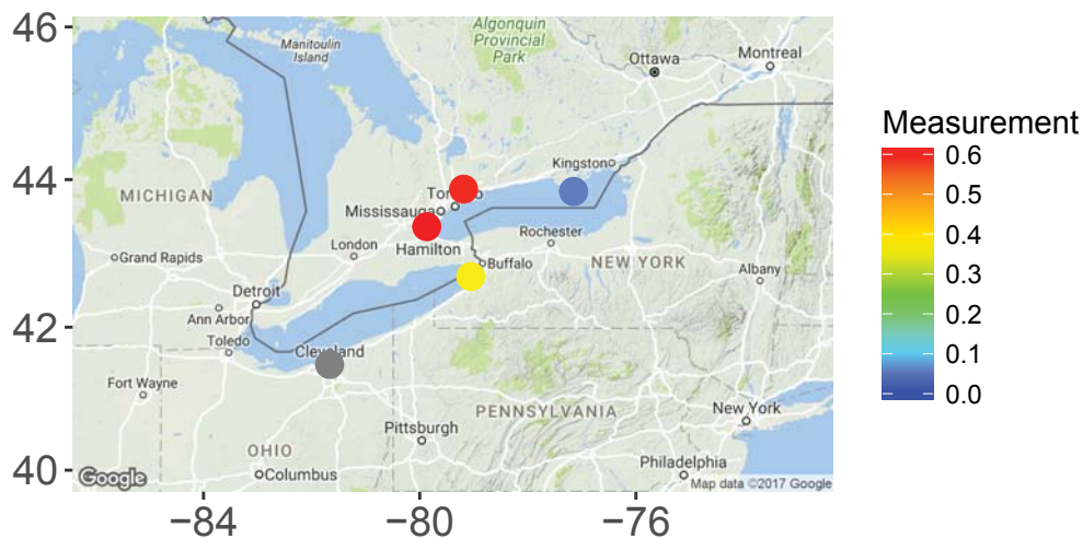
Measured wet deposition of PYR ( \mu\text{g m}^{-2} )
