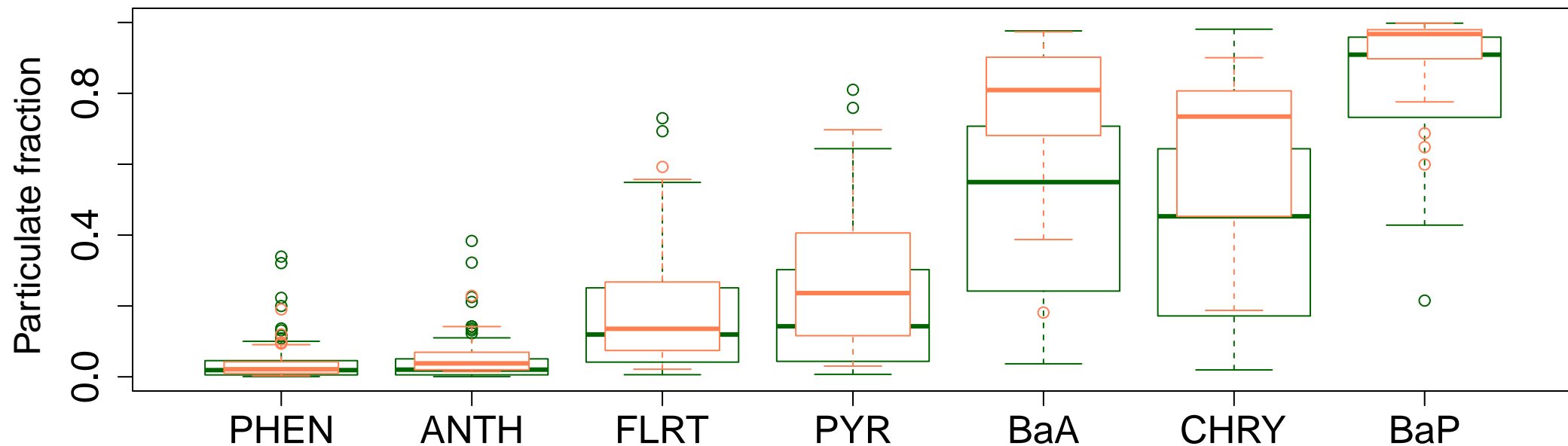
GEM-MACH-PAH modelled and measured particulate fraction, All IADN sites
