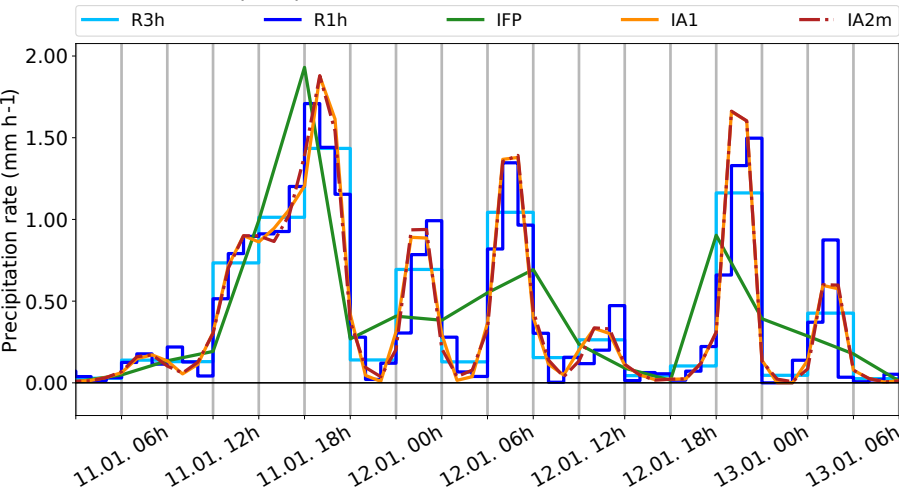
(b) Large-scale precipitation
