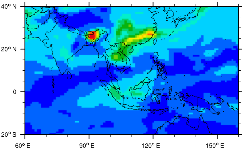
(c) MERRA2
