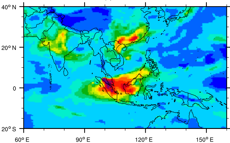
(c) MERRA2
