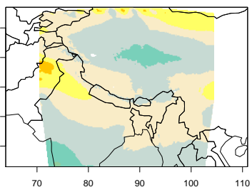
(e) WRF_ref_D01 May zonal wind
