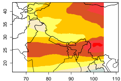
(b) ERA-Interim Feb zonal wind
