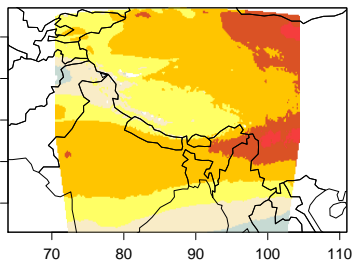
(a) WRF_ref_D01 Feb zonal wind
