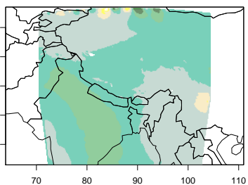
(g) WRF_ref_D01 May meridional wind
