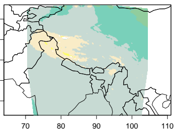
(c) WRF_ref_D01 Feb meridional wind
