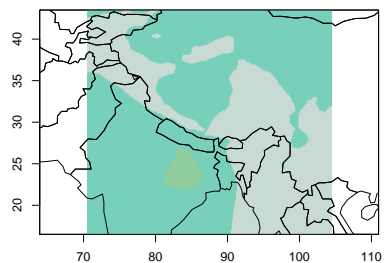
(h) ERA-Interim May meridional wind
