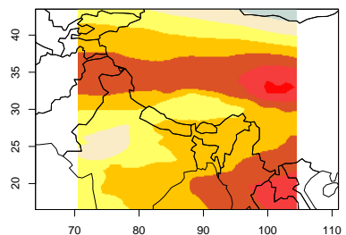
(f) ERA-Interim May zonal wind
