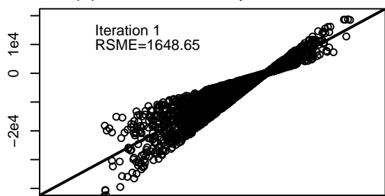
(a) Lanczos-CG optimization
