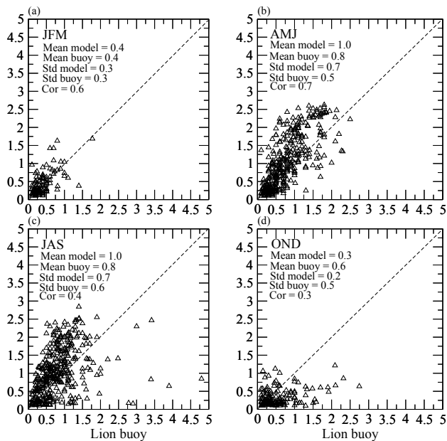
Figure 4. Amplitude in ^{\circ}\text{C} of the 2009–2013 SST diurnal cycle for the Lion buoy (x-axis) and the model simulation (y-axis), according to the season: (a) JFM, (b) AMJ, (c) JAS and (d) OND. Only values above 0.1^{\circ} are kept. Mean values and standard deviations are given for each season, as well as the daily temporal correlation.
