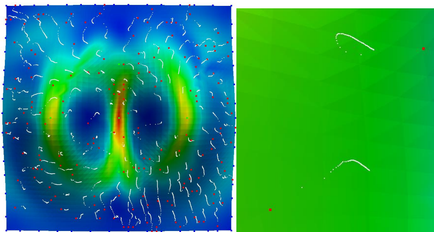
Figure 9. Trajectories of point convergences. The red points indicate the initial sample set, and the trajectories show the convergence trends, with closer gaps between candidate points. The right side shows a close view of the convergence of two points. These trends imply that the cCVT's convergence complies with Lloyd's relaxation linear convergence.
