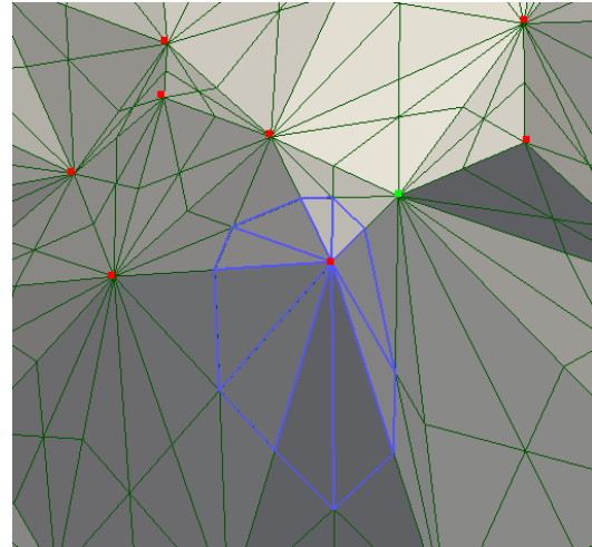
Figure 3. The triangles incident towards the first vertex r_i on the dual grid comprise an initial approximated Voronoi cell (rendered as a blue wireframe); the centre vertex is rendered in red.
