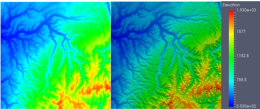
Figure 11. Experimental site 2: UTM11 Zone. Left: image view. Middle: hillshade view. It is a 3875 \times 3758 grid with a 10 m cell size.
