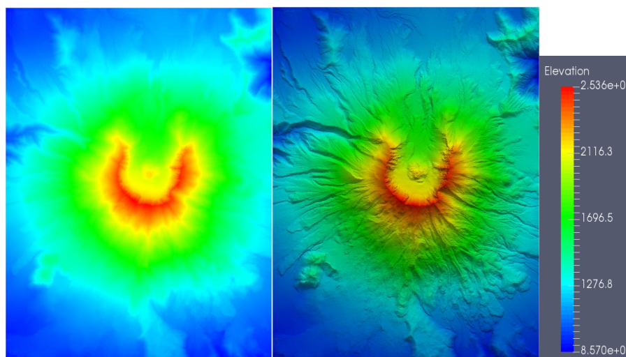
Figure 10. Experimental site 1: Mount St. Helens. Left: image view. Middle: hillshade view. It is a 2924 \times 3894 grid with a 3 m cell size.
