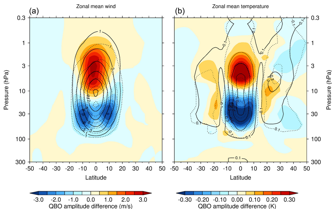
Figure 4. Comparison of Quasi-Biennial Oscillation amplitudes in u (a) and T (b) from models (solid contours) and reanalyses (dotted contours). The colours show the models–reanalyses difference, with blue depicting an underestimation by models and red an overestimation.
